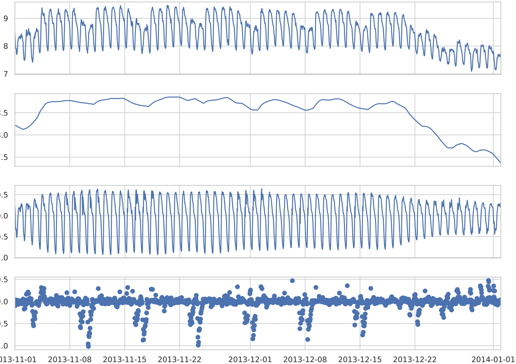
STL decomposition (period = 24 h) of \log(1+\text{business})
