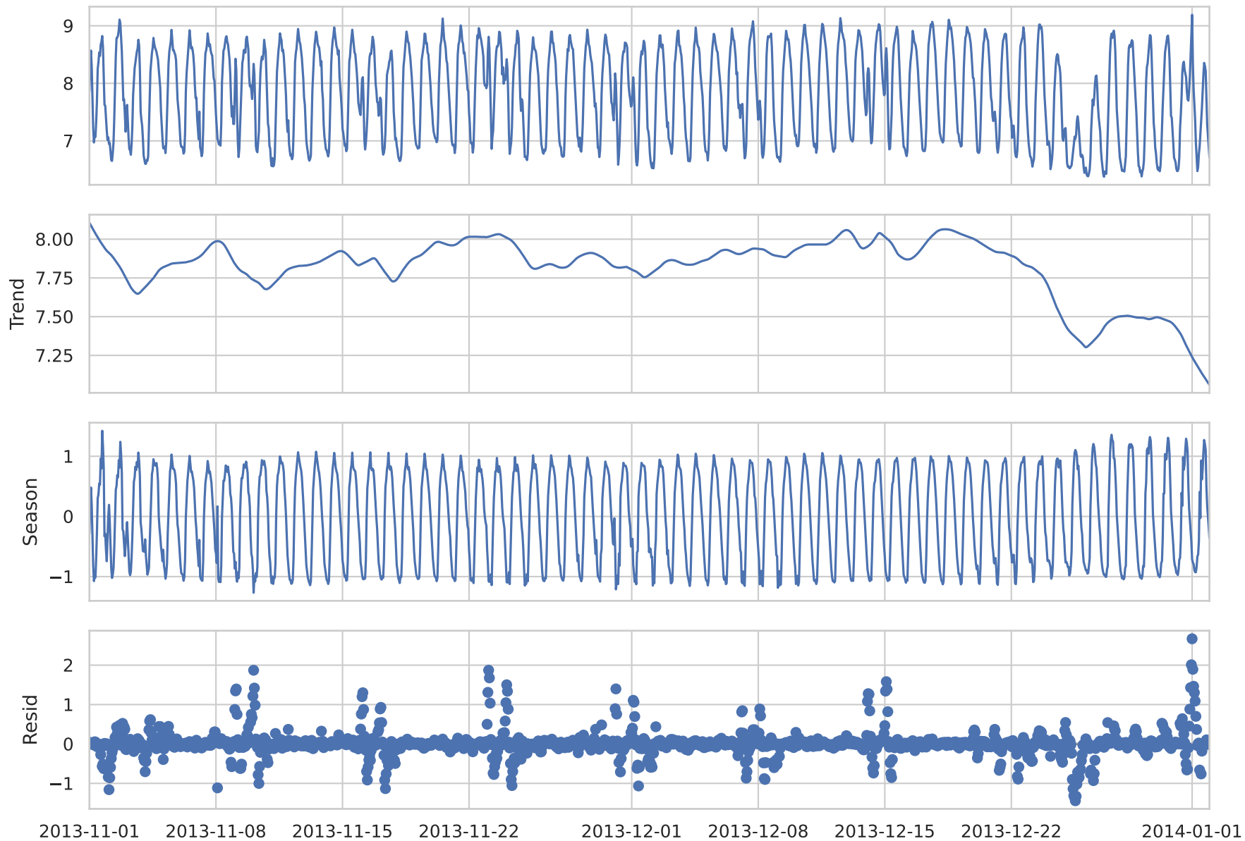
STL decomposition (period = 24 h) of \log(1+\text{duomo})
