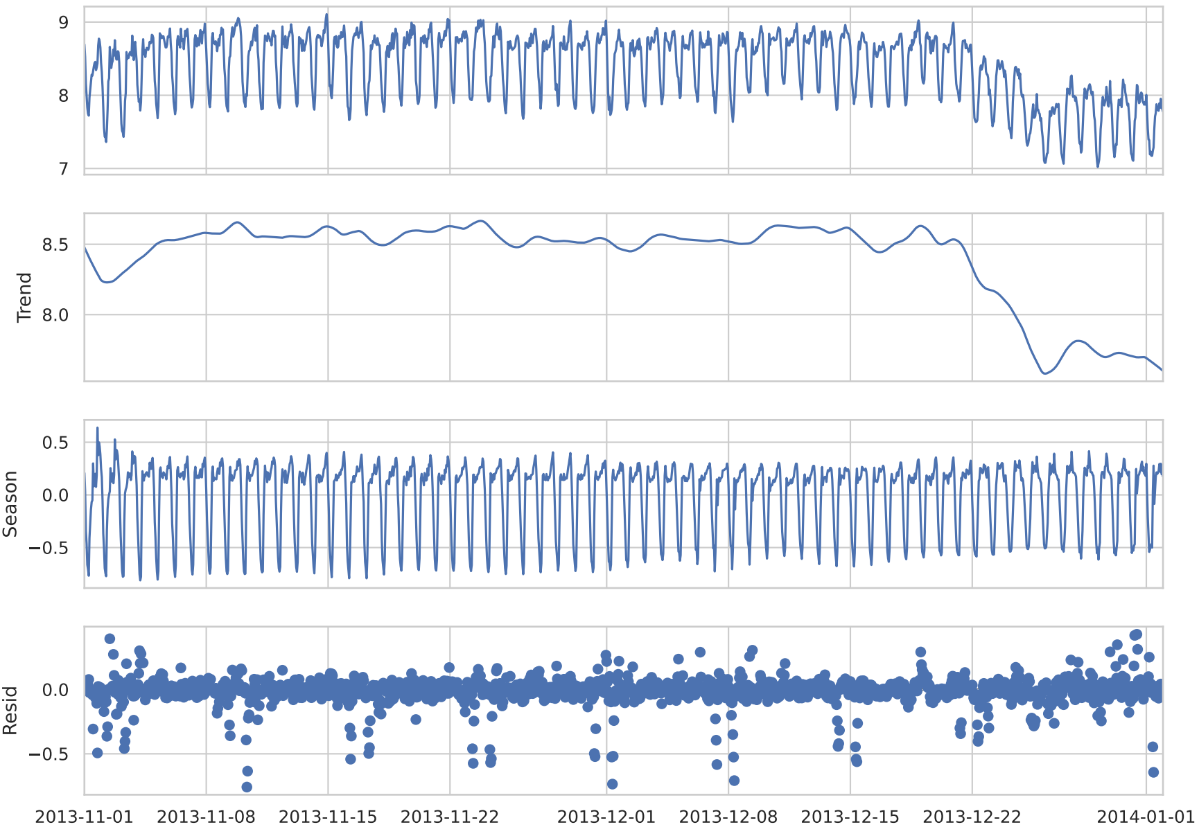
STL decomposition (period = 24 h) of \log(1+\text{mixed\_suburban}-2)
