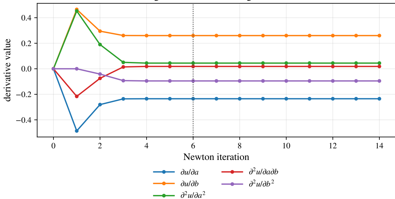
Convergence of selected design sensitivities
