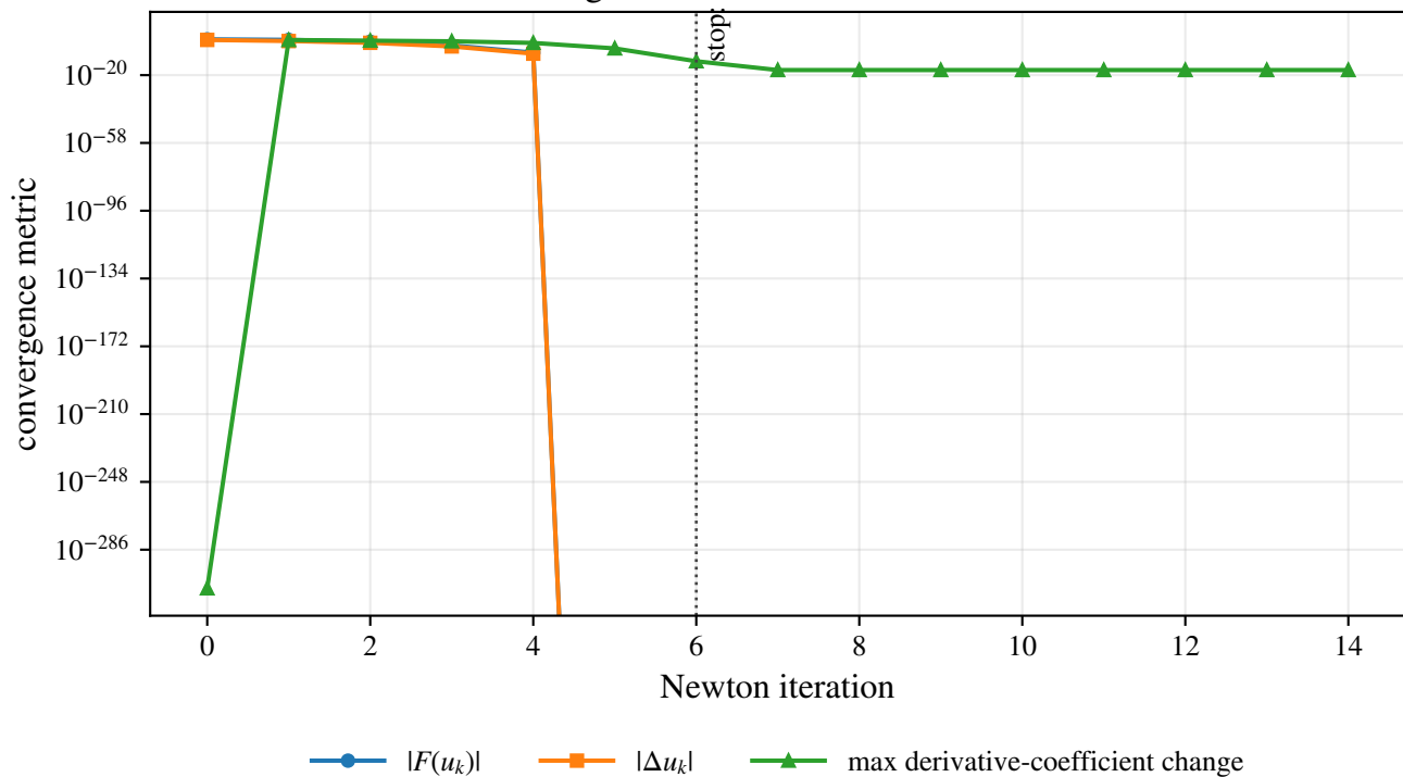
Newton convergence of state and derivative coefficients
