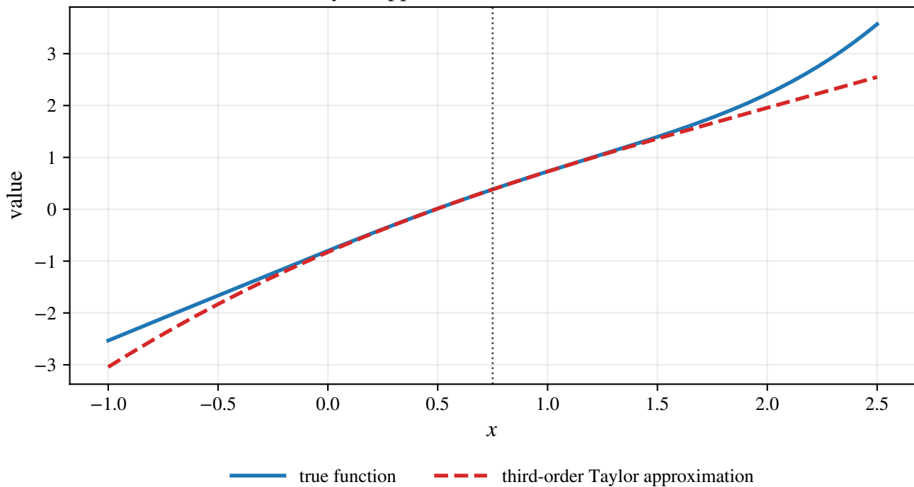
Local Taylor approximation from OTI coefficients
