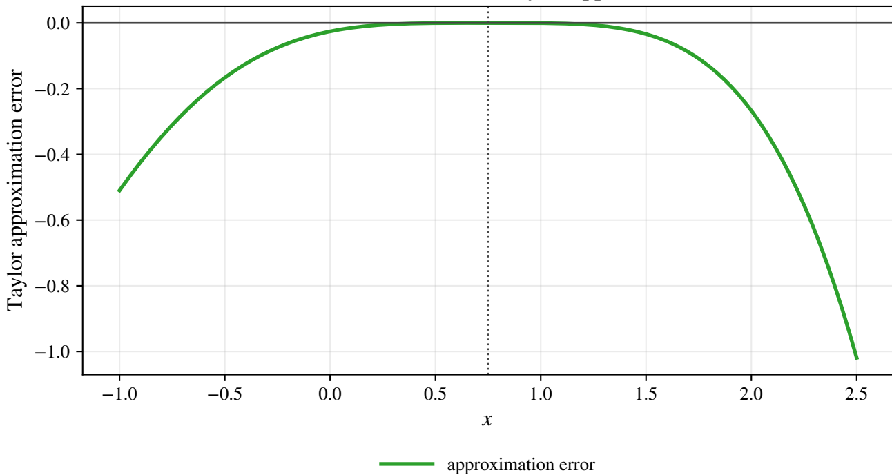
Error of third-order OTI Taylor approximation
