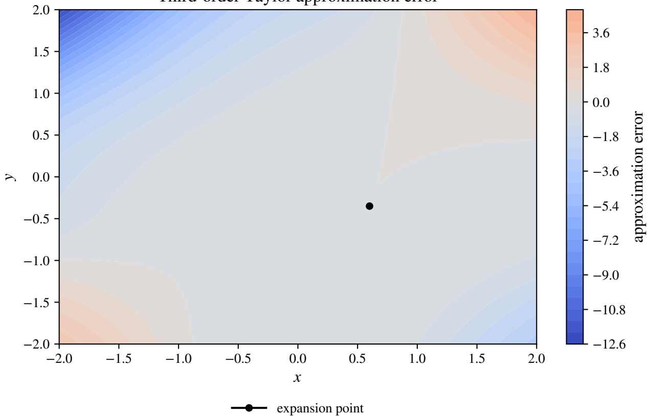
Third-order Taylor approximation error
