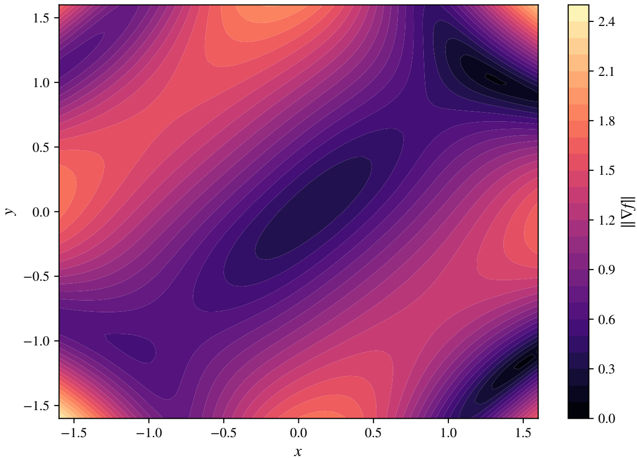
Three-dimensional scalar field slice, z_0 = 0.4
