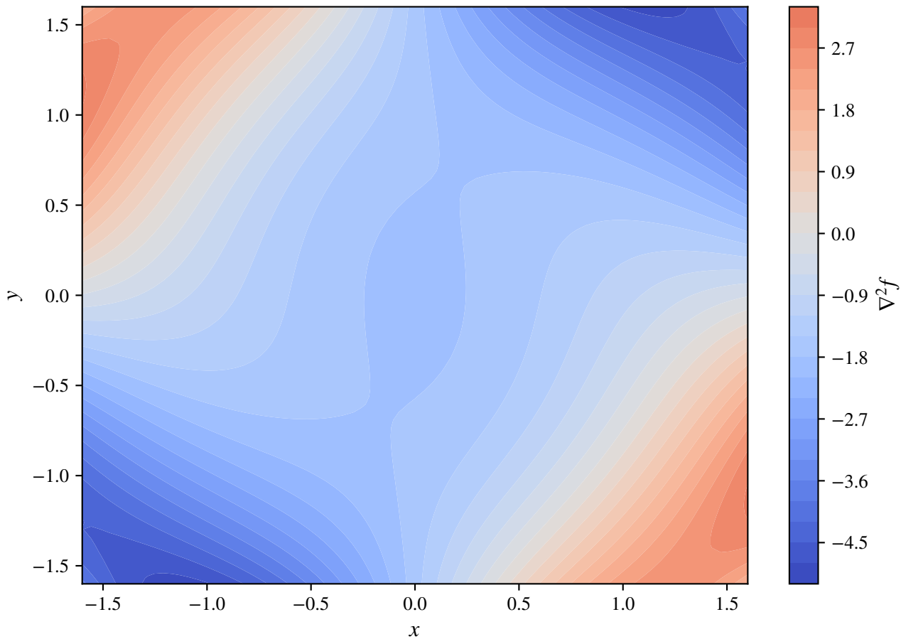
Three-dimensional scalar field slice, z_0 = 0.4
