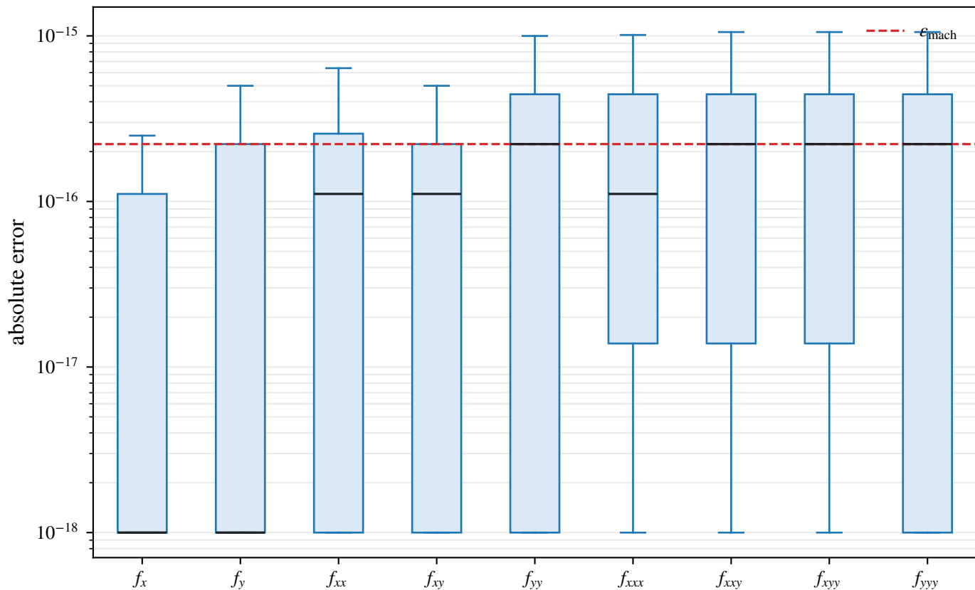
OTI derivative error over 1000 random evaluations
