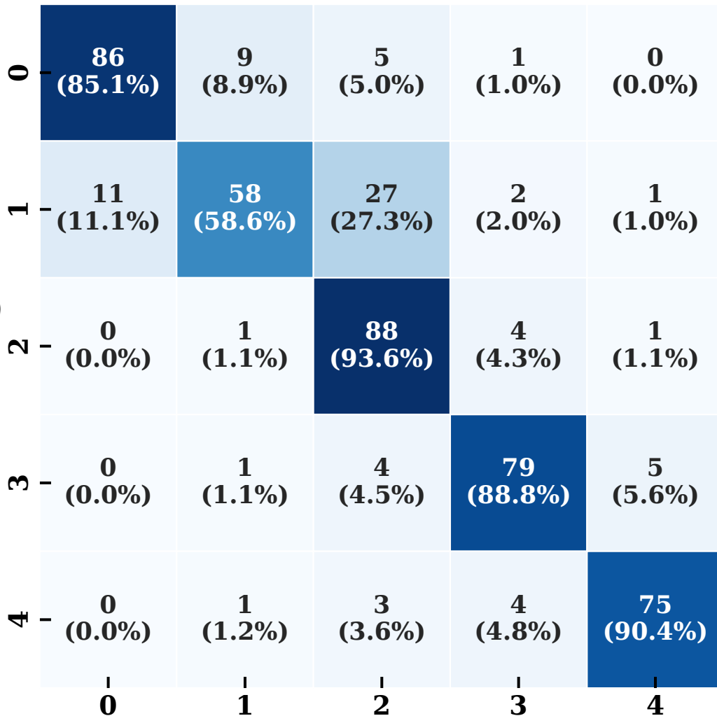
DenseNet121: confusion matrix (test)
