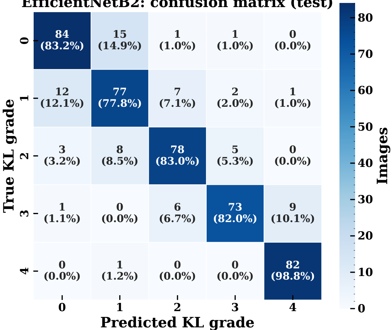
EfficientNetB2: confusion matrix (test)
