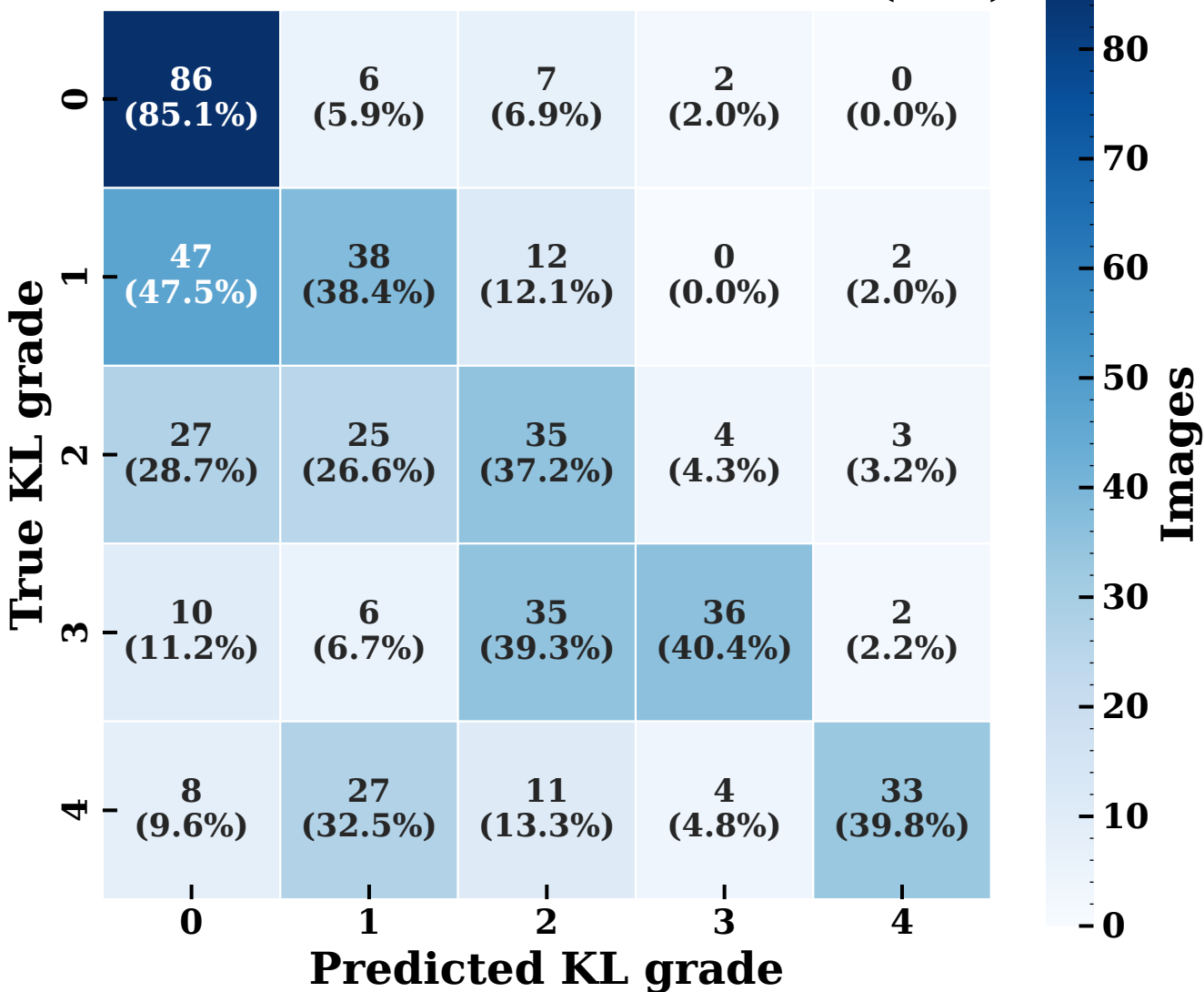
DenseNet121: confusion matrix (test)
