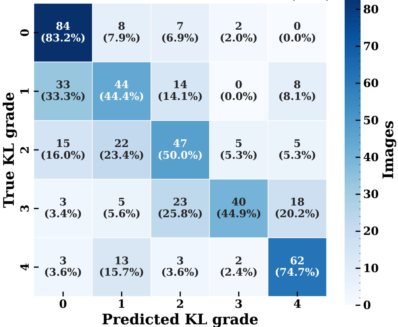
DenseNet201: confusion matrix (test)
