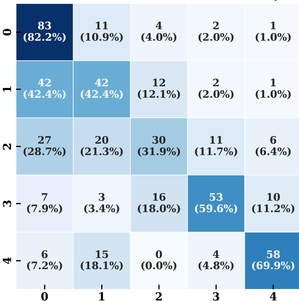
EfficientNetB0: confusion matrix (test)
