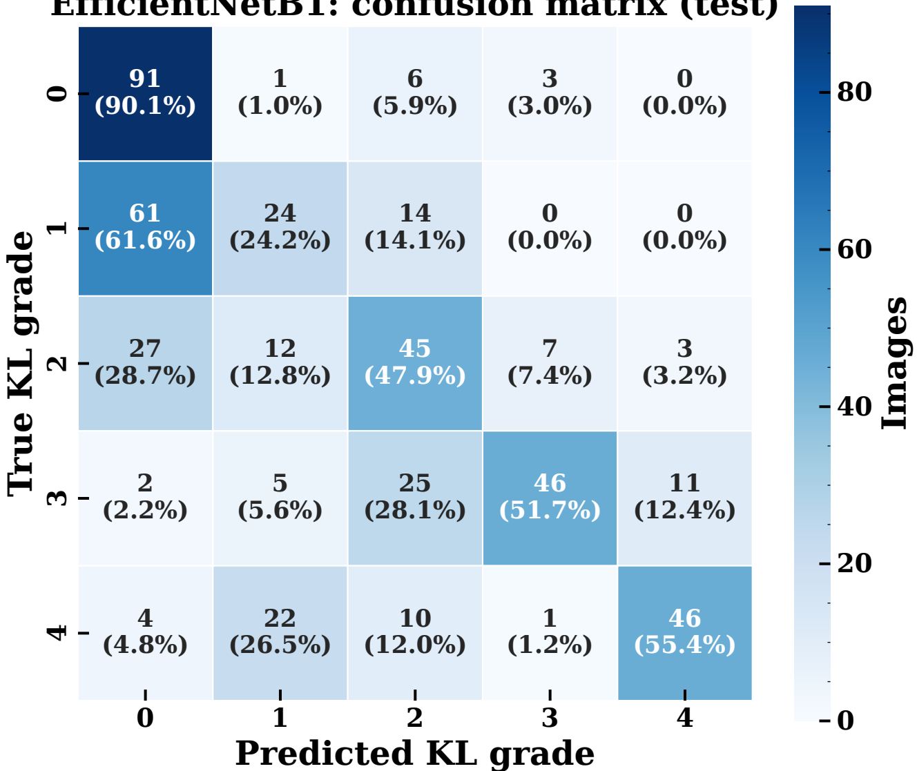
EfficientNetB1: confusion matrix (test)
