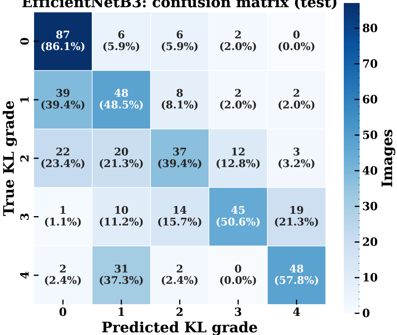
EfficientNetB3: confusion matrix (test)
