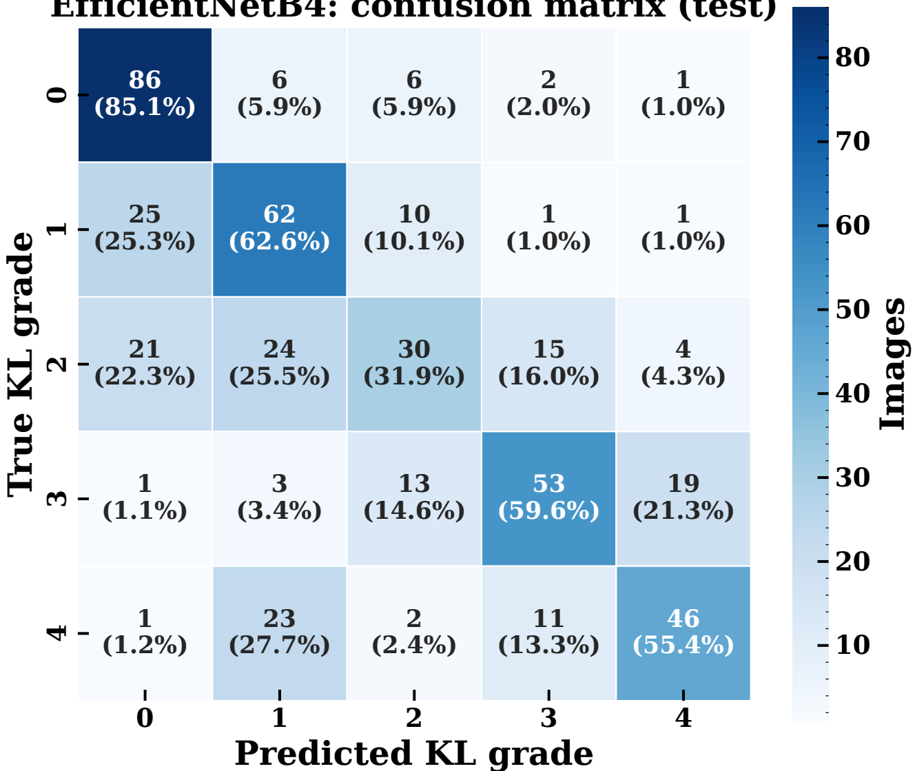
EfficientNetB4: confusion matrix (test)
