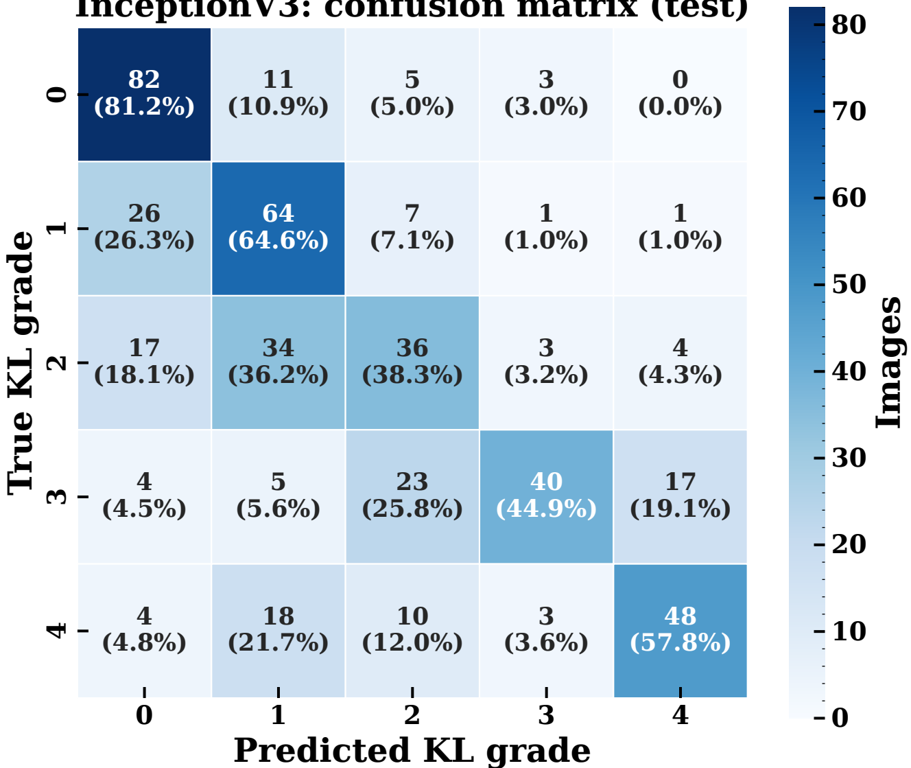
InceptionV3: confusion matrix (test)
