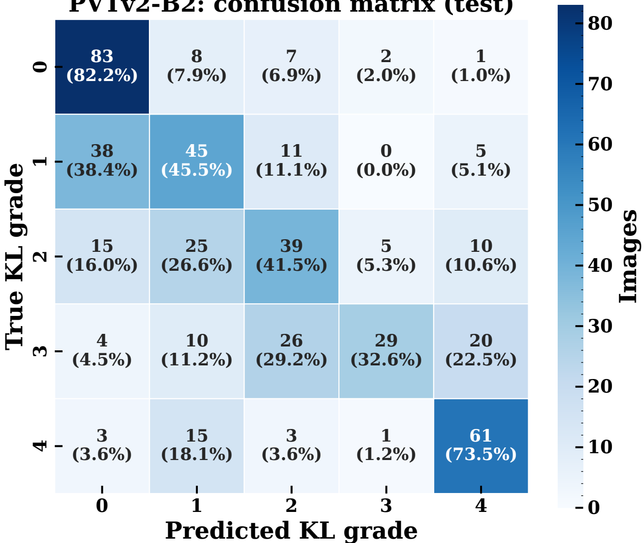
PVTv2-B2: confusion matrix (test)
