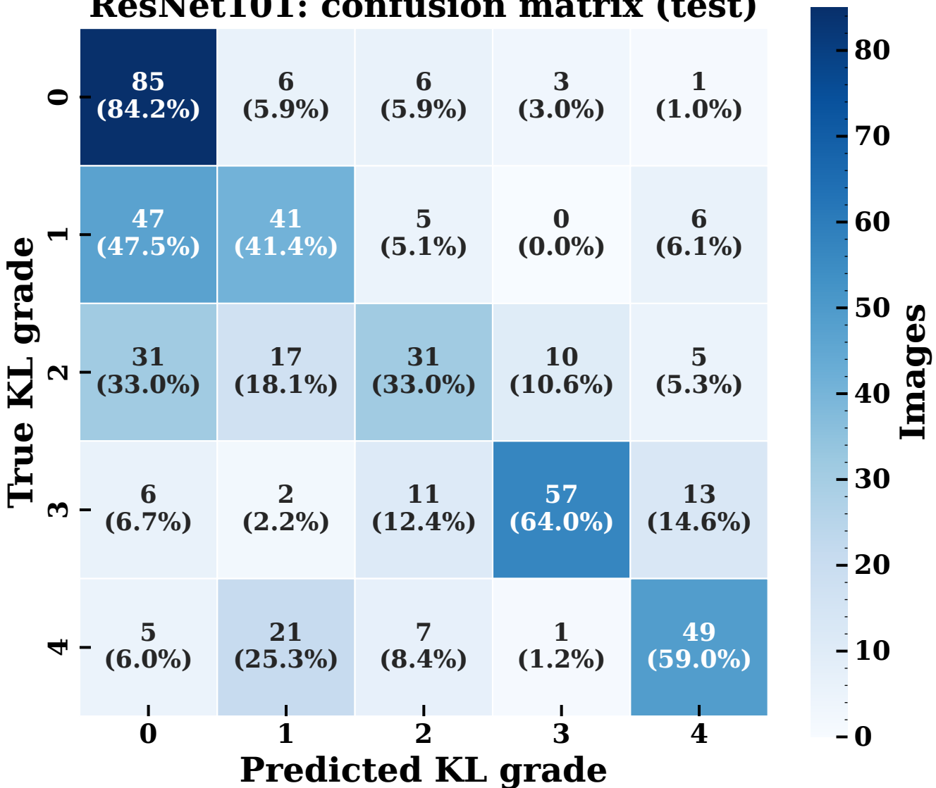
ResNet101: confusion matrix (test)
