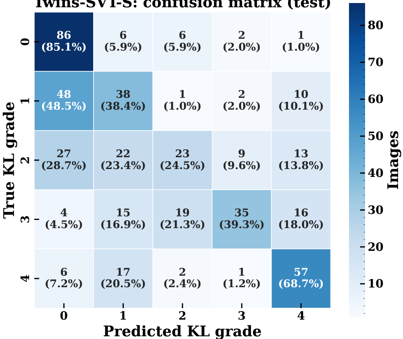
Twins-SVT-S: confusion matrix (test)
