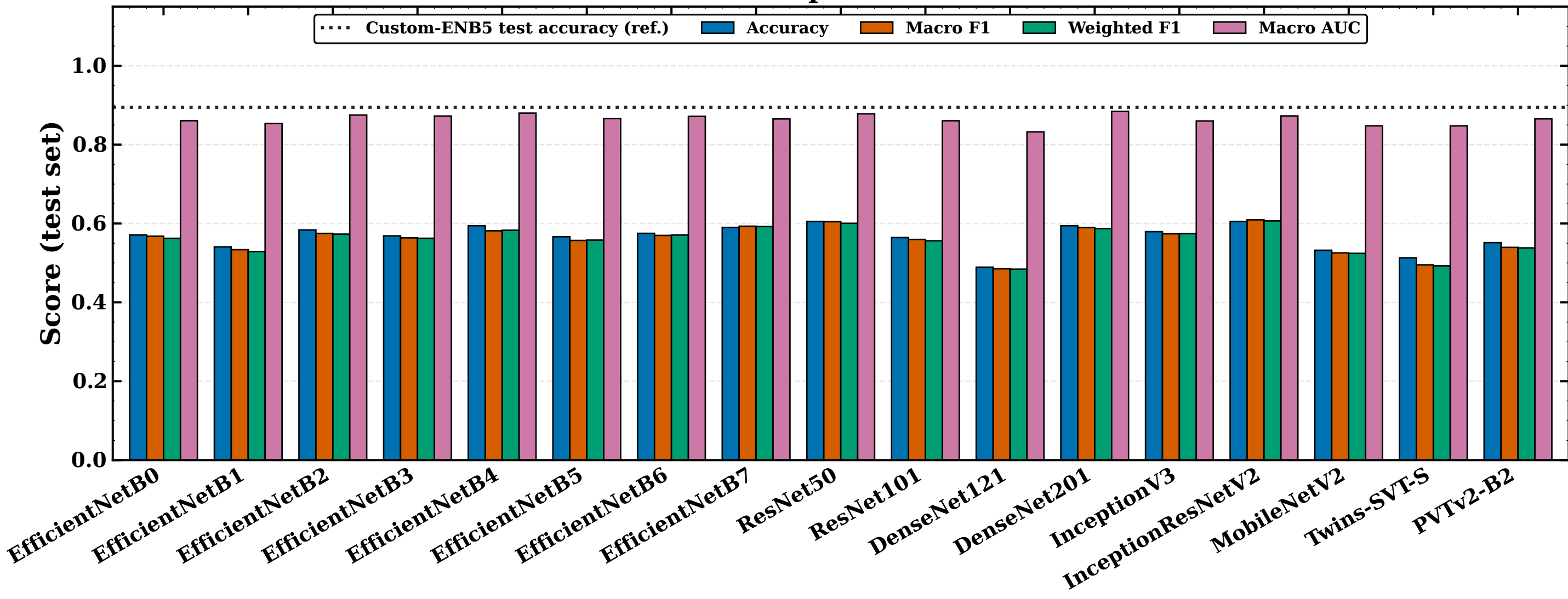
Test-set performance
