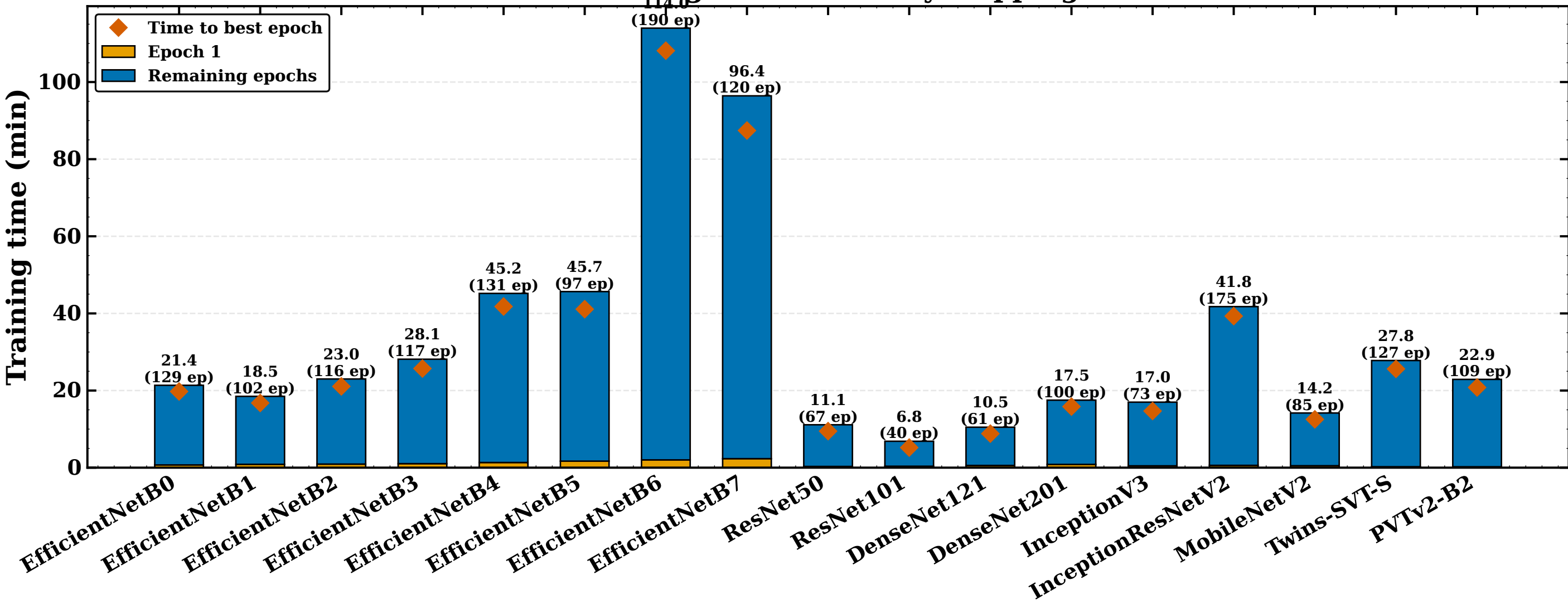
Training time with early stopping
