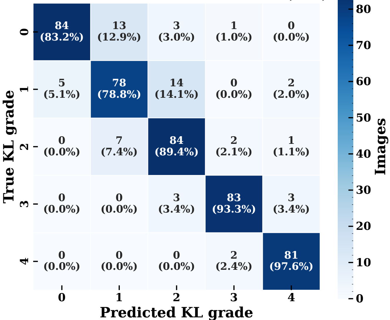
Custom-ENB5: confusion matrix (test)
