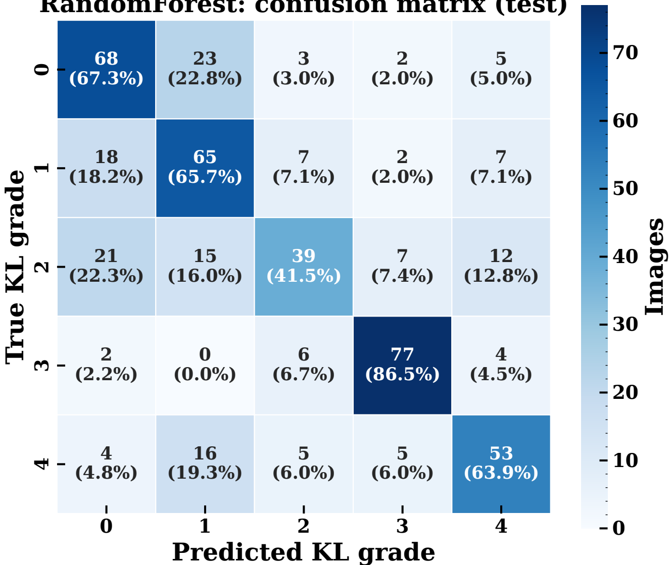
RandomForest: confusion matrix (test)
