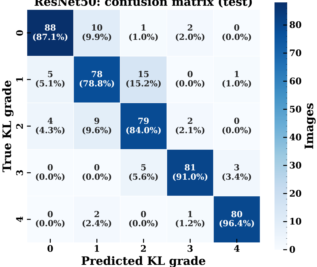
ResNet50: confusion matrix (test)
