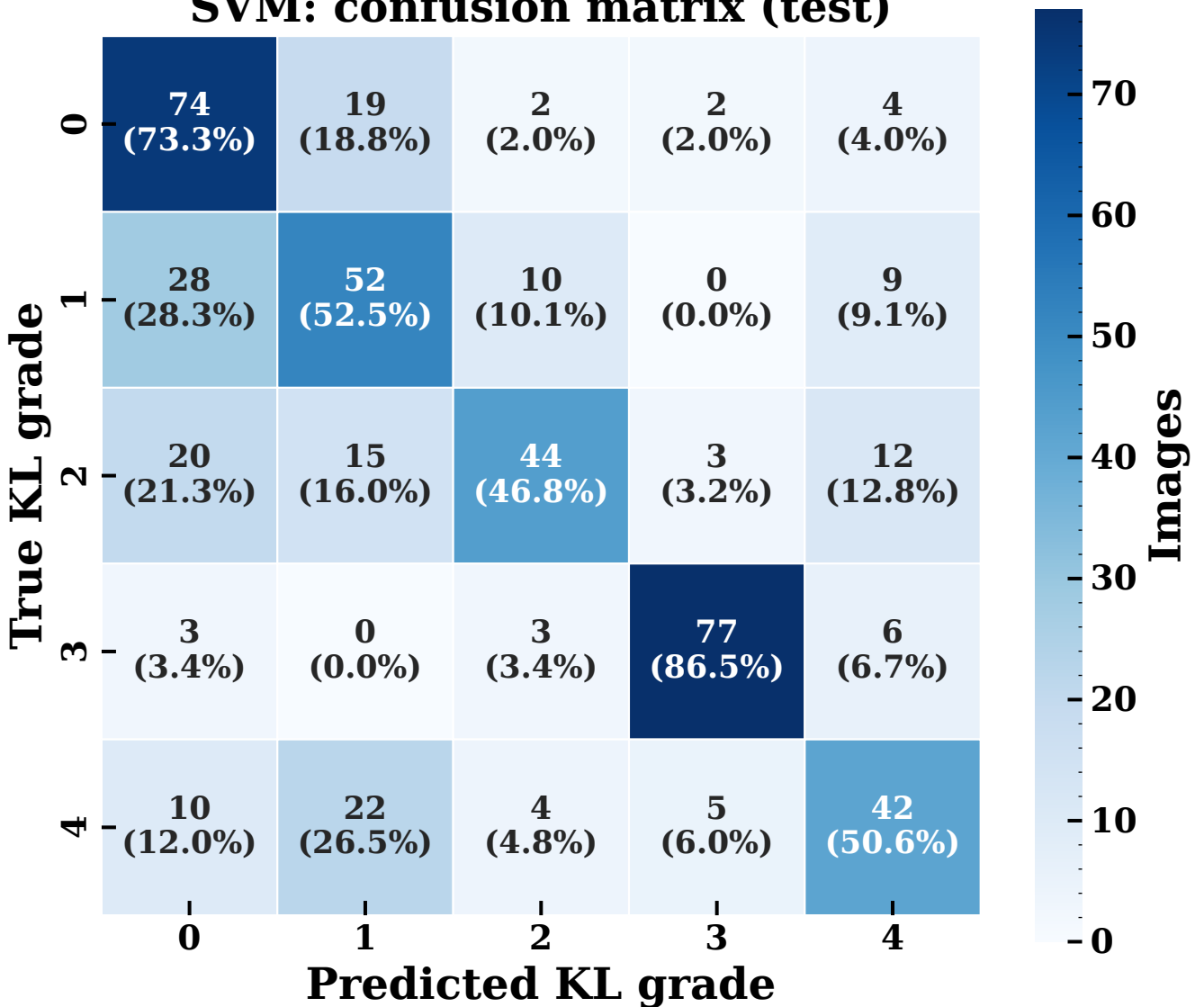
SVM: confusion matrix (test)
