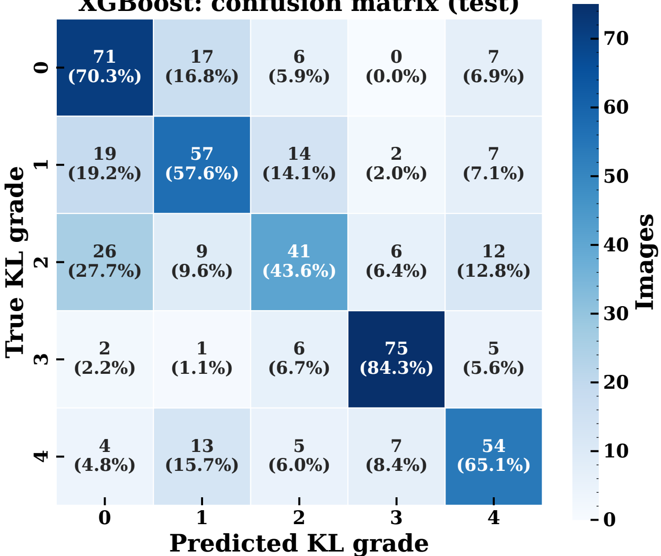
XGBoost: confusion matrix (test)
