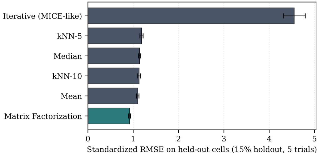
Imputation method comparison
