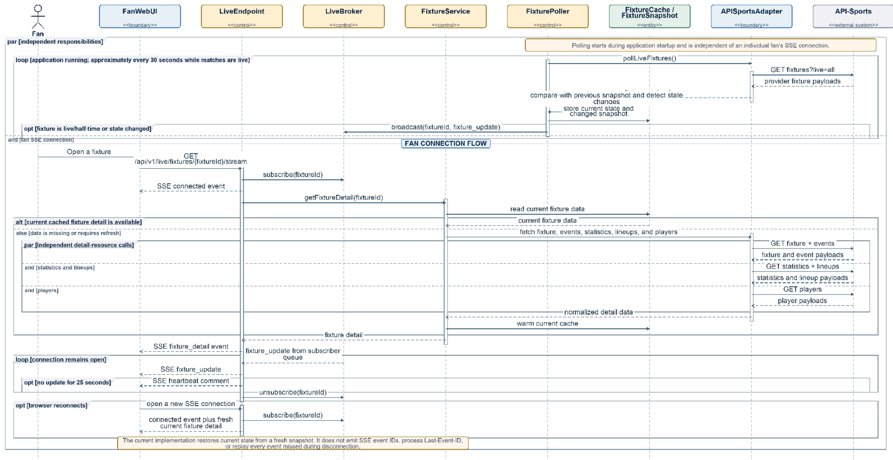
Figure 1. UML sequence diagram for view live match updates.
