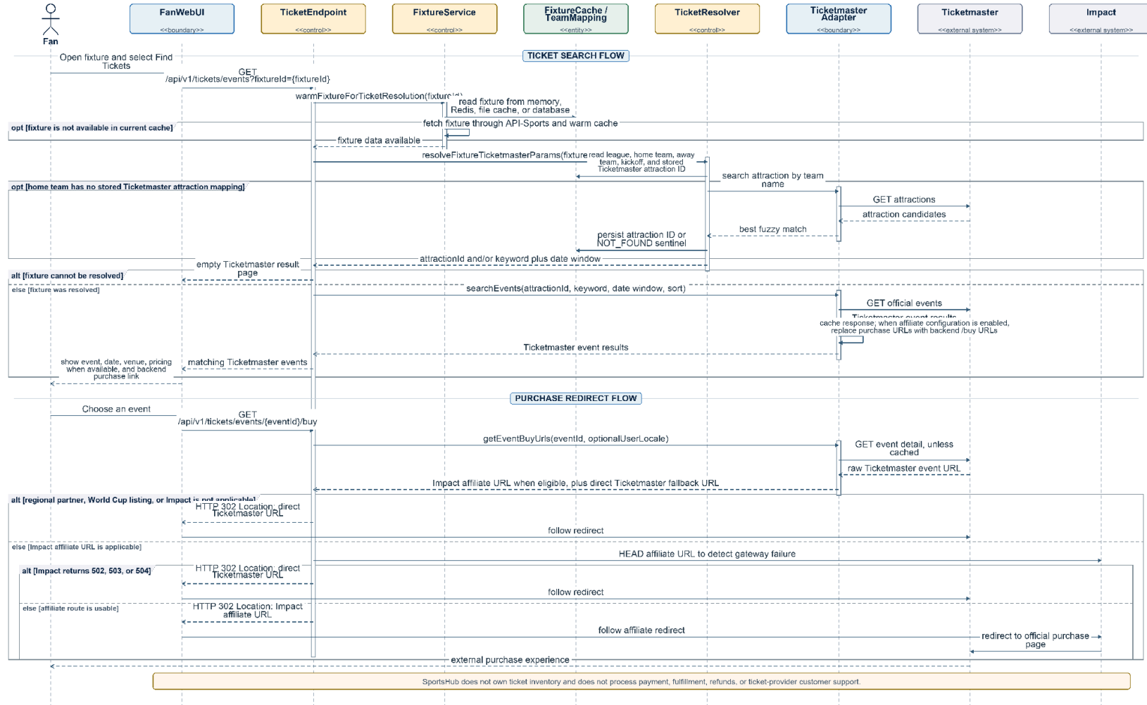
Figure 3. UML sequence diagram for discovering official tickets.
