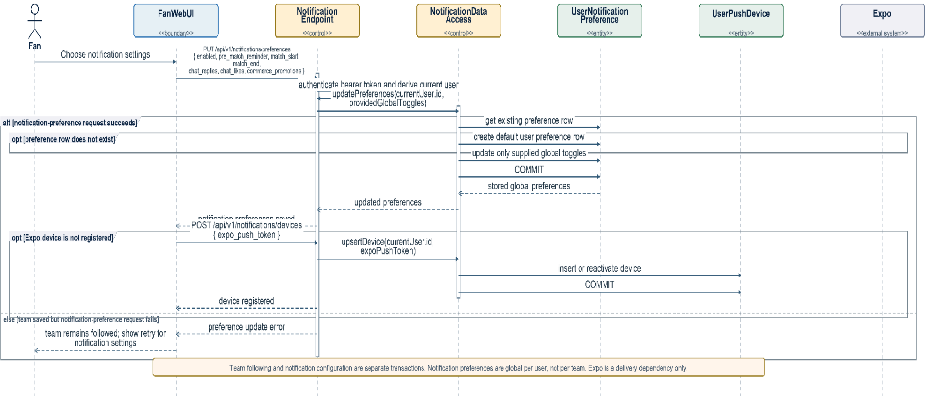
Figure 2B. UML sequence diagram for configuring notification preferences and push delivery.
