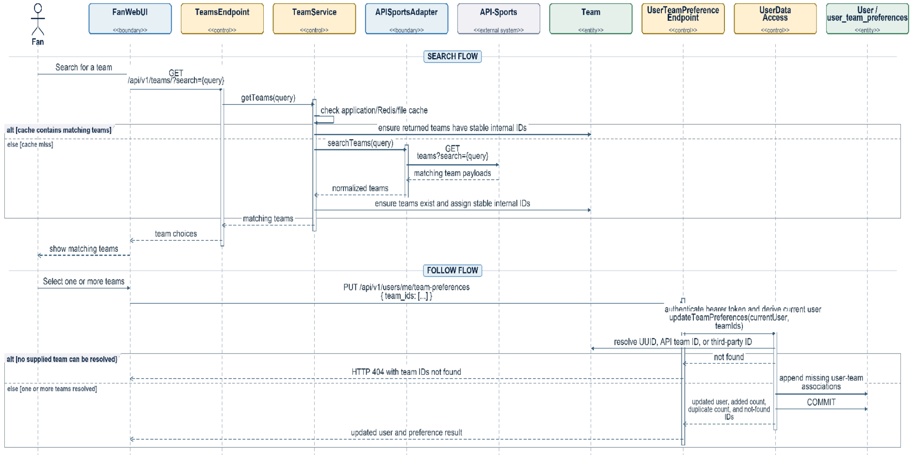
Figure 2A. UML sequence diagram for searching for and following a team.
