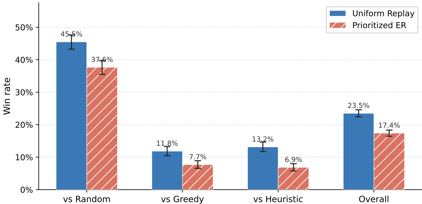
DQN Win Rate vs Baseline Opponents (1 000 games per pair; error bars: 95% bootstrap CI)
