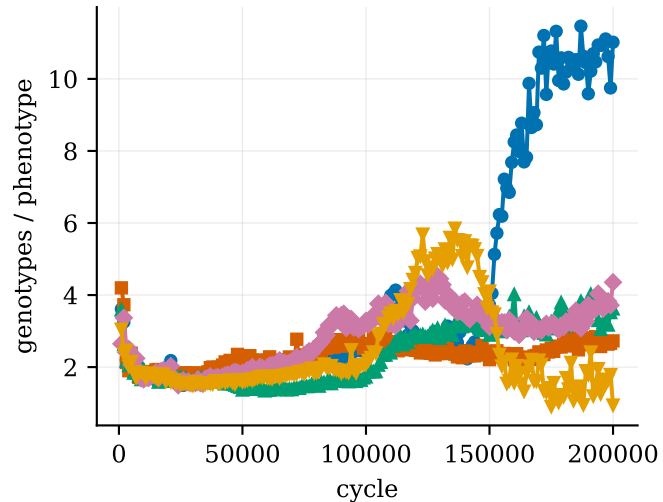
GP-map redundancy
