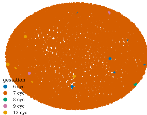
Genotype network (edges=1--2 mutations, colour=speed)
