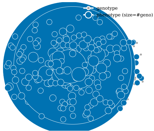
Bipartite genotype \leftrightarrow phenotype (seed 62, cycle 200000)
