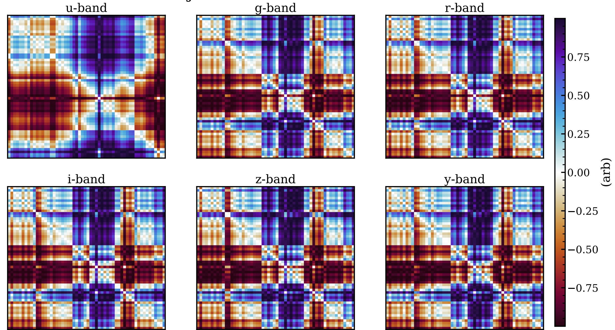
Object ID: 71676 - Class: AGN
