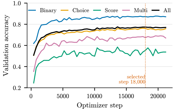
(b) Validation accuracy (3,000 examples)
