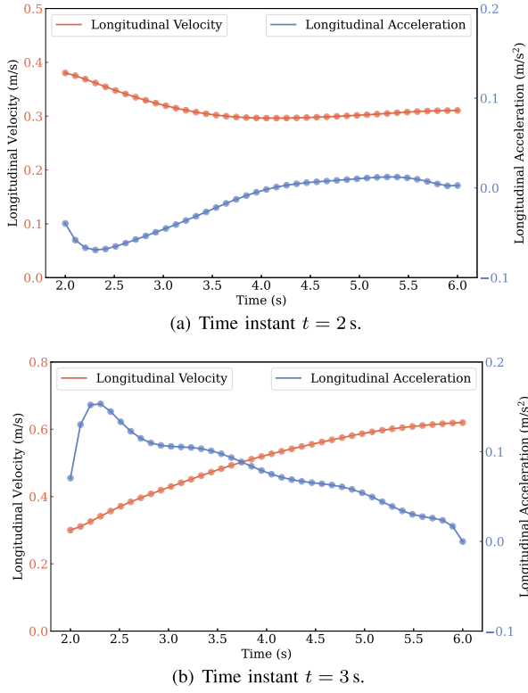
Fig. 8. Optimal longitudinal velocity and acceleration profiles of the selected trajectory at two different time instants. (a) EV decelerates as it approaches the occluded intersection. (b) EV accelerates to pass through the intersection.
