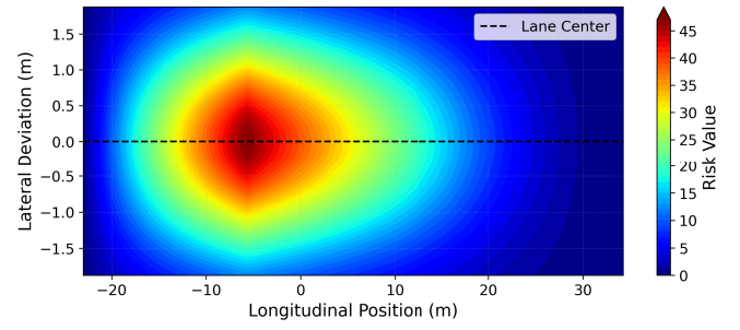
Fig. 2. Spatial distribution of risk around EV in the presence of occlusion. The EV is positioned at [0, -2 \text{ m}] , with the occluded area extending from [-8, 0 \text{ m}] to [-2, 0 \text{ m}] . The quantitative color scale (right), labeled “risk value,” illustrates the risk level, where warmer colors (e.g., red) represent higher risk and cooler colors (e.g., blue) indicate lower risk.
