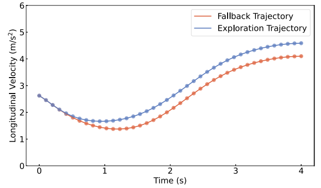
Fig. 5. Generated velocity profiles of two trajectories at time instant 7 s. Two trajectories show the shared initial segment and the separate process for safe navigation.
