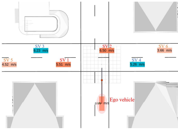
Fig. 3. Top-down view of the EV navigating through a dynamic and occluded intersection under dense traffic conditions. The blue vehicles (SV3, SV4) represent noninteracting vehicles whose future trajectories do not intersect with EV. The lighter orange vehicles (SV5, SV6) are occluded, while the solid orange vehicles (SV1, SV2) are fully visible. The EV plans two potential trajectories to manage the occlusion risks: the black exploration trajectory prioritizes travel efficiency, while the conservative fallback trajectory accounts for higher occlusion risks.
