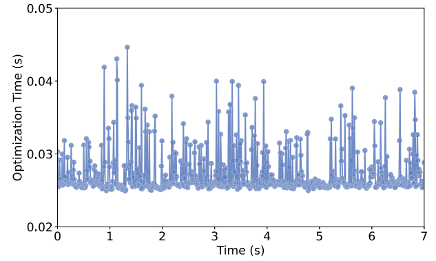
Fig. 9. Evolution of the optimization time with a prediction step of N = 40 while interacting with three SVs. The average and maximum optimization time are 27.33 and 44.65 ms, respectively.
