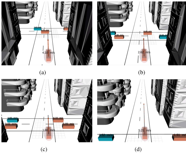
Fig. 4. Third-person view snapshots of the red EV navigating through a dense and occluded intersection at different time instants. The proposed occlusion-aware contingency planner enables EV to first decelerate to avoid potential hazards and then accelerate to safely pass through the occluded intersection under dense traffic conditions. (a) Time instant t = 5.5 s. (b) Time instant t = 7 s. (c) Time instant t = 9.9 s. (d) Time instant t = 12.5 s.
