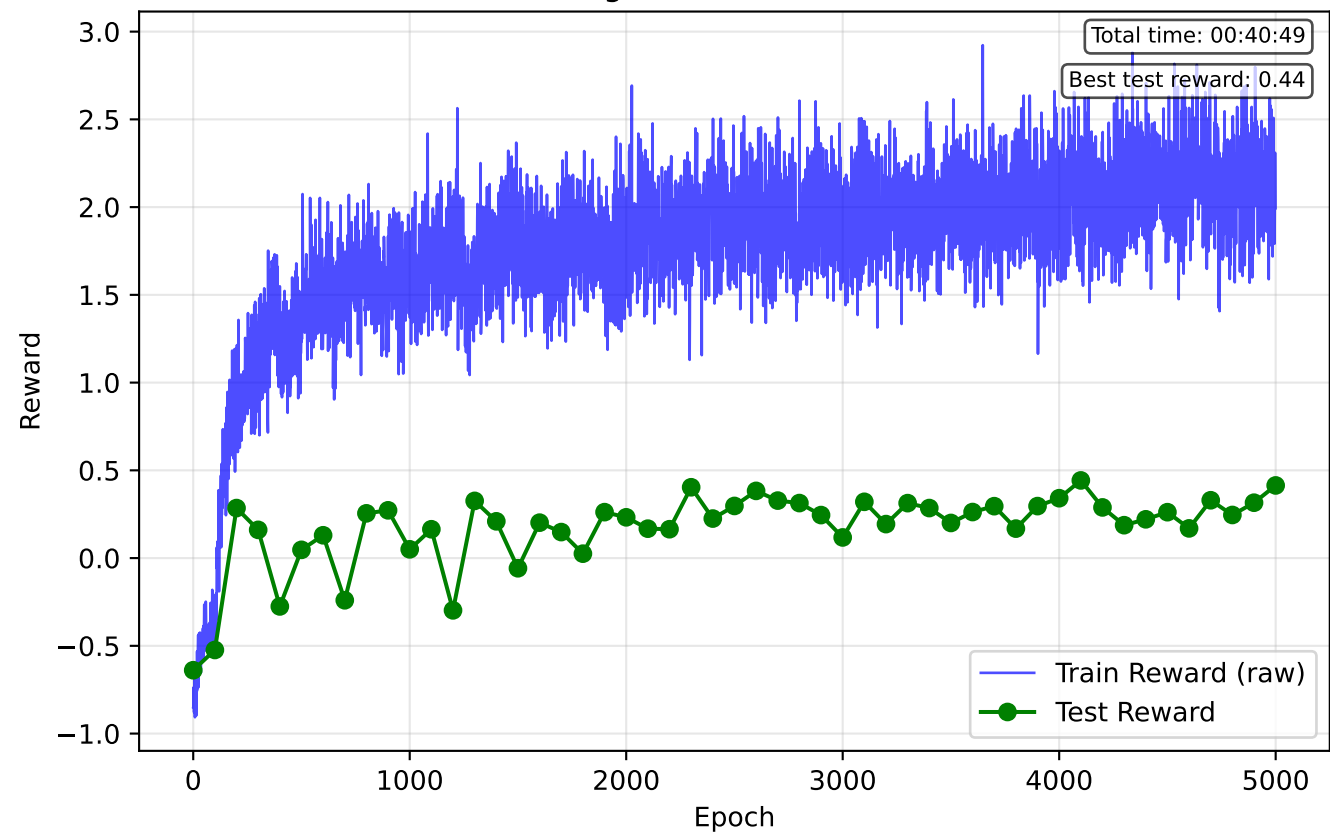
Training & Test Rewards (raw)
