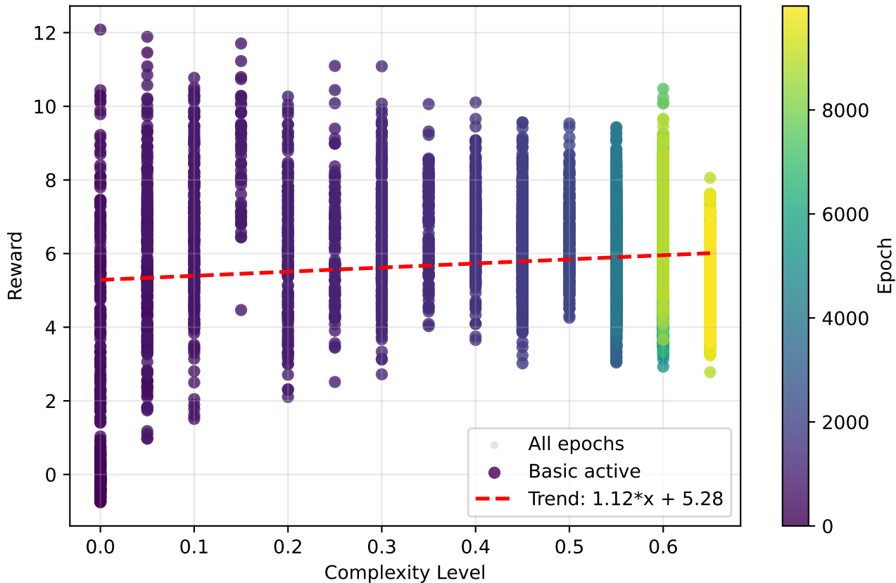
Reward vs Complexity - Basic stage (raw data)
