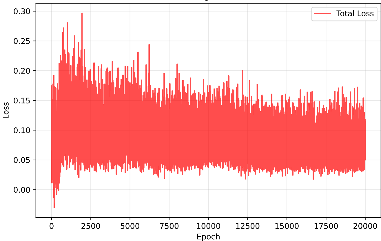
Training Losses
