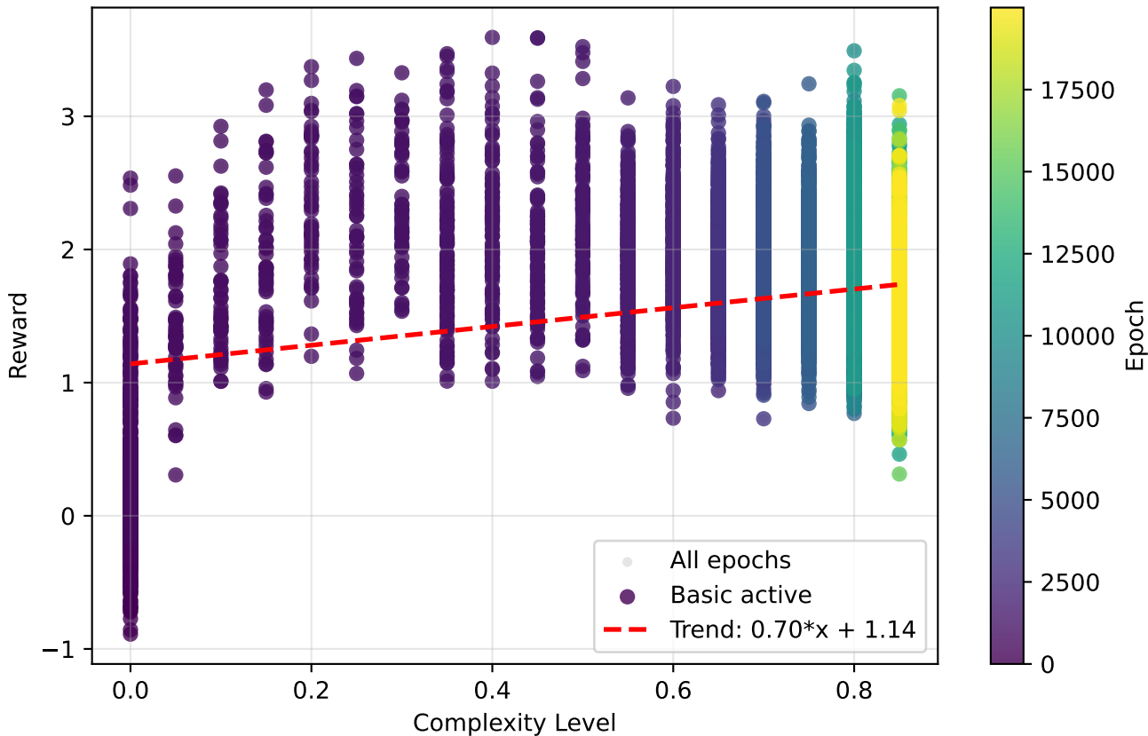
Reward vs Complexity - Basic stage (raw data)
