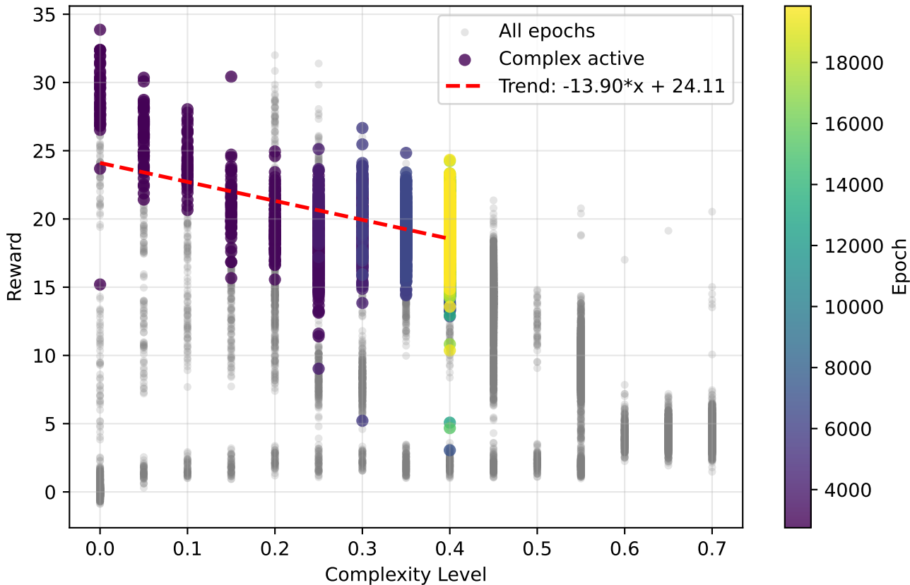
Reward vs Complexity - Complex stage (raw data)
