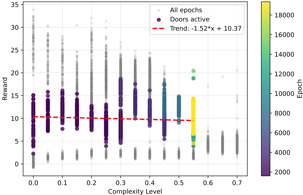
Reward vs Complexity - Doors stage (raw data)
