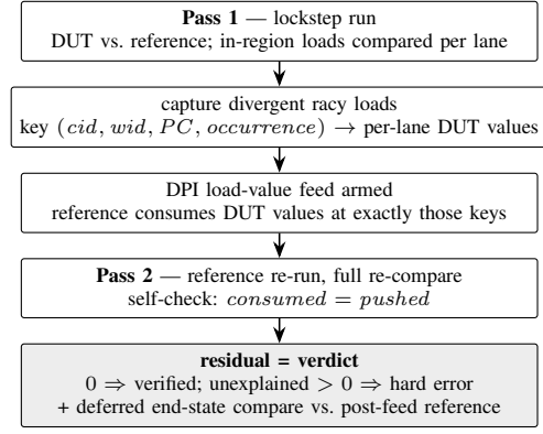
Fig. 2. The two-pass load-value feed. Only captured racy loads are fed; every other divergence in pass 2 remains an error, so the mechanism cannot mask a DUT bug.
