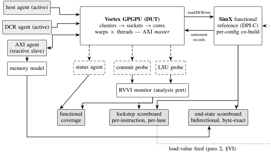
Fig. 1. Environment architecture. Solid gray boxes are active UVM agents; dashed boxes are passive probes (never checkers); dark boxes are the two verdict-rendering scoreboards and coverage. The DUT is the bus master; stimulus is a compiled program in the memory model.
