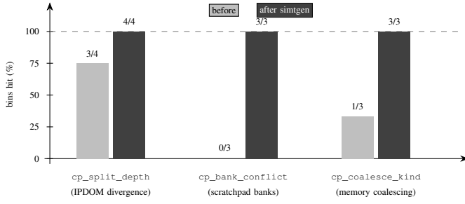
Fig. 3. Effect of axis-directed generation on the three open SIMT coverage targets (bins hit, as a percentage of the coverpoint’s bin count). Before simtgen (light bars): depth-4 IPDOM divergence was unreachable by any of 50 random-program seeds (3/4 bins); bank conflicts never occurred in 70,498+ sampled cycles (0/3—its root-caused to a coverpoint-definition defect, since the crossbar admits one winner per bank per cycle); one coalescing class was unhit (1/3). Deliberate divergence-tower and bank-hostile kernels (dark bars) closed all three to 100%. Measured in isolated merges; a full-suite re-run folding these into the frozen topology banks is documented as pending, so the headline totals of Table III do not yet include them.
