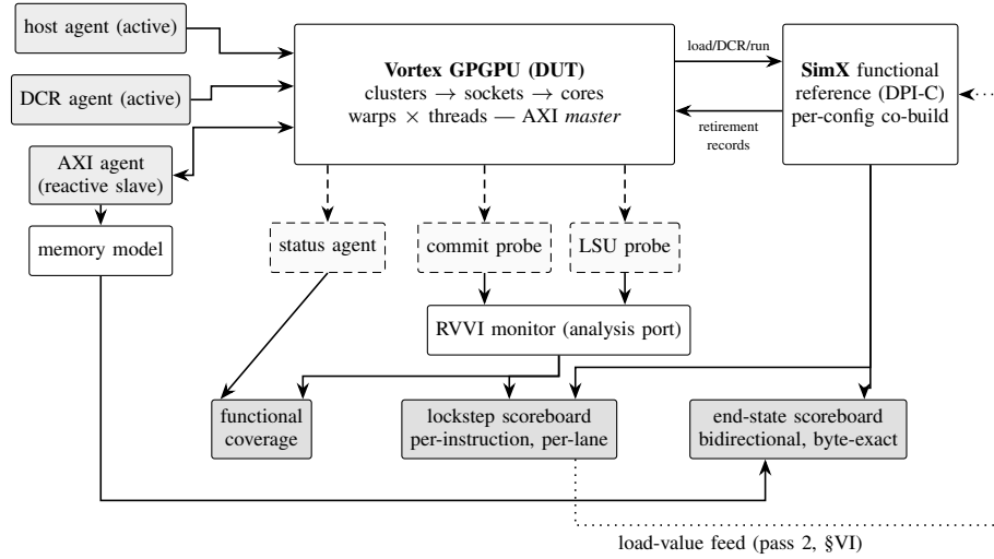
Fig. 1. Environment architecture. Solid gray boxes are active UVM agents; dashed boxes are passive probes (never checkers); dark boxes are the two verdict-rendering scoreboards and coverage. The DUT is the bus master; stimulus is a compiled program in the memory model.
