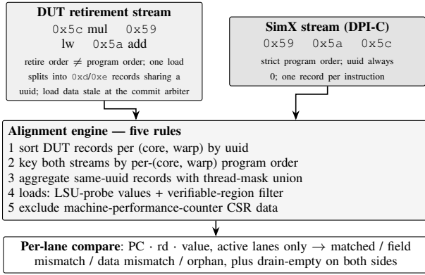
Fig. 2. The lockstep alignment pipeline. The DUT stream (left) carries the SIMT quirks that a scalar-CPU RVVI flow never meets; the reference stream (right) is strictly ordered. Each rule removes exactly one class of false mismatch: sorting fixes out-of-order retirements (Rule 1), program-order keying bridges the reference’s null uuids (Rule 2), mask-union aggregation reassembles split loads (Rule 3), the LSU probe with region filter restores sound load comparison (Rule 4), and volatile-CSR exclusion removes timing-only divergences (Rule 5). After alignment, any remaining difference outside the three declared exception classes is a real defect.
