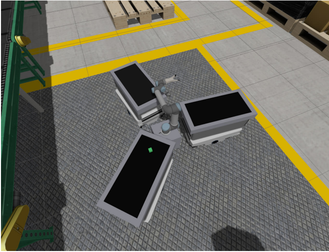
Fig. 7. Twin execution of the optimized winner val_0: the UR5 + RG2 arm reaches into a conveyor station mid-relay. The three stations are pinwheeled around the arm in the optimizer’s chosen layout; the welded part (green cube) is carried between stations. Both trials complete the full pick–place–pick–place relay with no planning failures (Table VIII).
