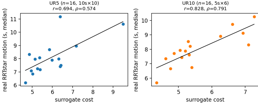
Fig. 6. Surrogate vs. real RRTstar motion time at scale ( n = 16 per robot, median estimator). The surrogate correlates with real motion on both arms (UR5 full planning budget, UR10 reduced budget); fit lines and bootstrap statistics in Table VII.
