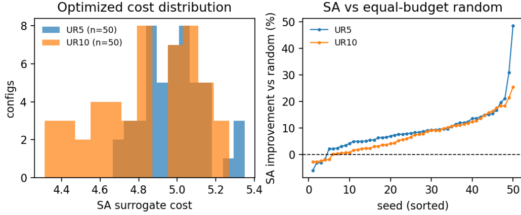
Fig. 5. Generalization across 50 seeds and two arms. Left: optimized-cost distribution for UR5 and UR10. Right: per-seed improvement of simulated annealing over the equal-budget random baseline (sorted); SA beats random on 46/50 (UR5) and 45/50 (UR10) seeds.
