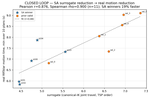
Fig. 3. Pooled surrogate vs. real motion ( n = 11 ). Optimized winners (low end) and random valids lie on the same trend; the surrogate reduction maps onto a real-motion reduction.
