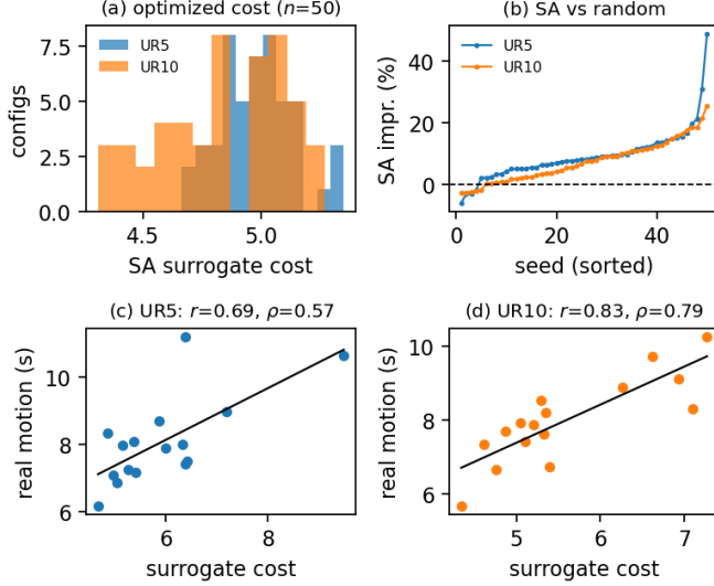
Fig. 5. Generalization across 50 seeds and two robot arms. (a) Optimized-cost distribution. (b) Per-seed improvement of simulated annealing over the equal-budget random baseline; SA wins 46/50 (UR5) and 45/50 (UR10). (c,d) Surrogate vs. real RRTstar motion at scale ( n = 16 , median estimator) for UR5 (full planning budget) and UR10 (reduced budget); fit lines shown, bootstrap statistics in Table VII.
