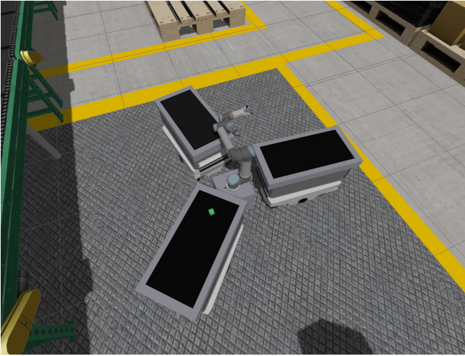
Fig. 6. Twin execution of the optimized winner val_0: the UR5 + RG2 arm reaches into a conveyor station mid-relay. The three stations are pinwheeled around the arm in the optimizer’s chosen layout; the welded part (green cube) is carried between stations. Both trials complete the full pick–place–pick–place relay with no planning failures (Table VIII).
