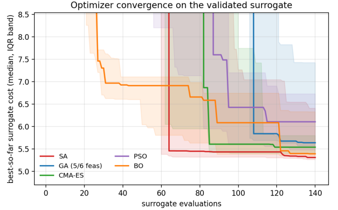
Fig. 4. Convergence of the five optimizers on the validated surrogate (median best-so-far over six seeds, IQR band). The top three converge to a statistically indistinguishable cost; random placement never enters the feasible band.
