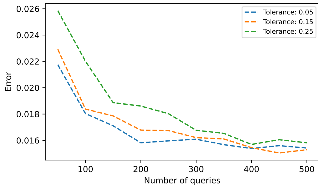
Learning error for haar-random unitaries, Distr = haar, n = 6
